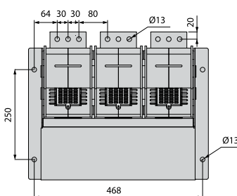
3200A Bottom View
