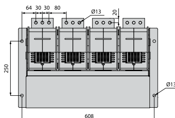
3200A Bottom View
