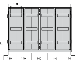
3200A Back View
